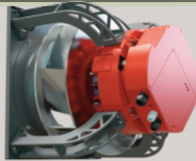
Direct Drive Backward Curved Airfoil Plenum Fan with Infinitum Aircore EC Motor
