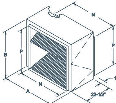
F9200A FILTER SECTION For Model 9200 Duct Blowers
