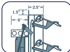
SERIES 3200M OUTWARD MOUNT
