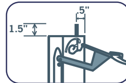
SERIES 3100 INWARD MOUNT
