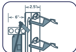
SERIES 3000M SIDE MOUNT - NO FLANGE
